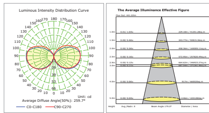
10W GLOW BAR 38205-019
