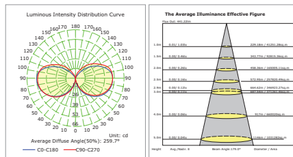
10W GLOW BAR 38205-019
