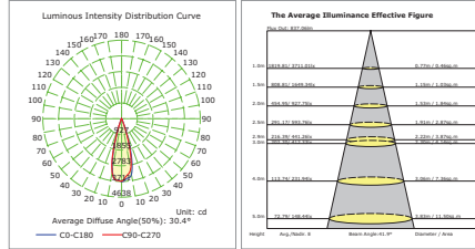
13W ADJUSTABLE SPOT LIGHT 38141-010
