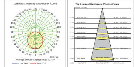
10W FIXED DOWN LIGHT 38142-017
