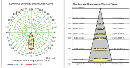
8W ADJUSTABLE SPOT LIGHT 38140-013
