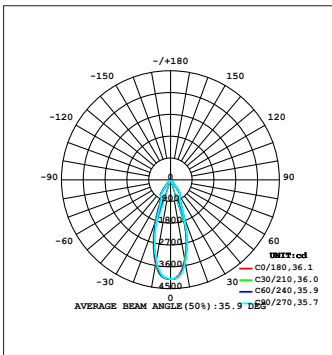
30W SPOT
