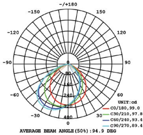
15W 1-LIGHT WALL WASH CLEAR
