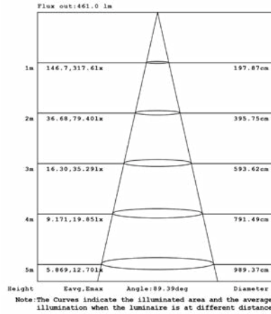
15W 1-LIGHT WALL WASH CLEAR
