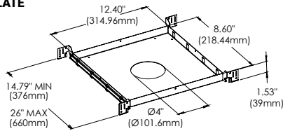
CUT HOLE: Trim & Trimless: Ø4"
